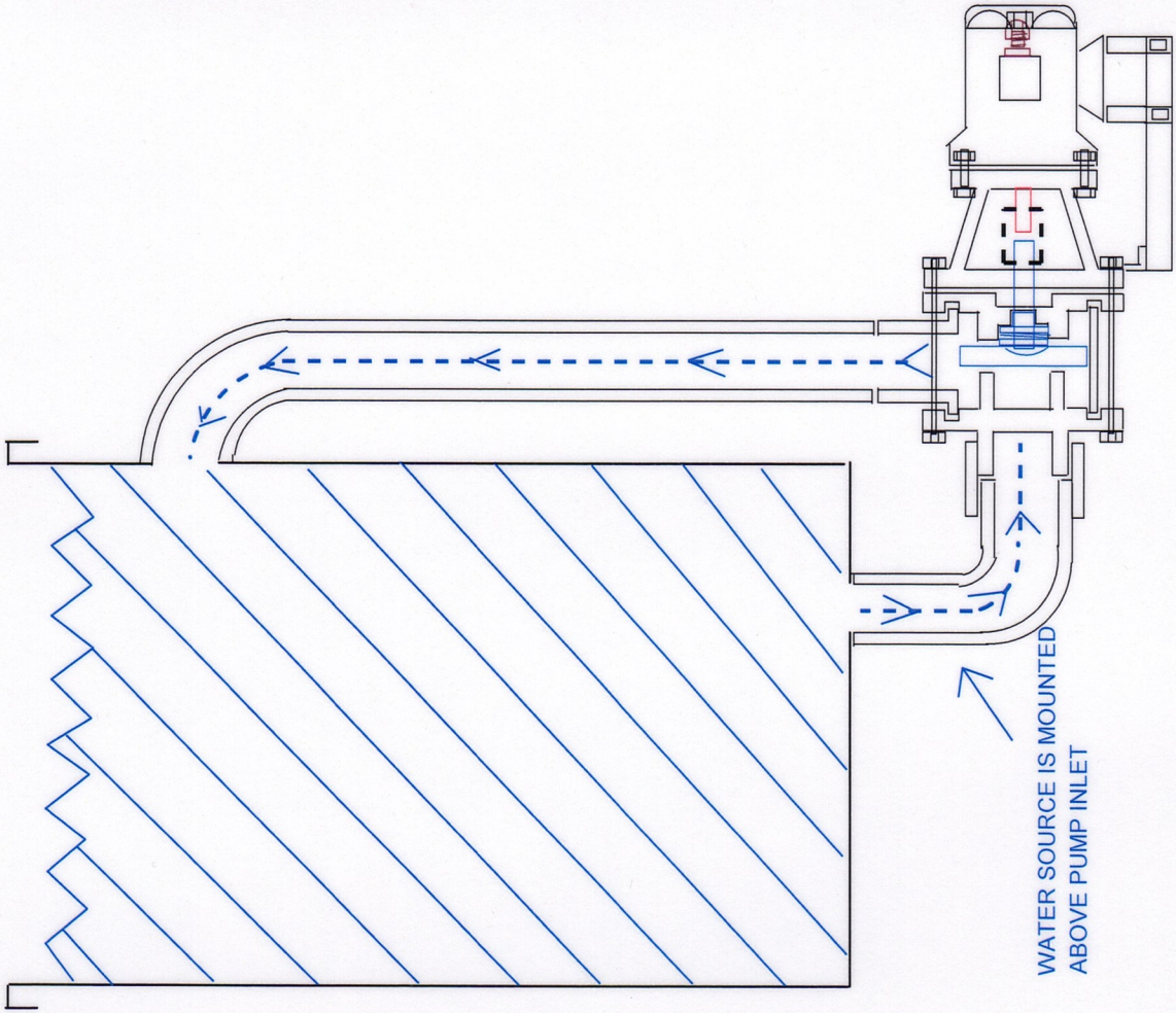
EXAMPLE OF FLOODED SUCTION IDEAL INSTALLATION METHOD FOR PUMP
